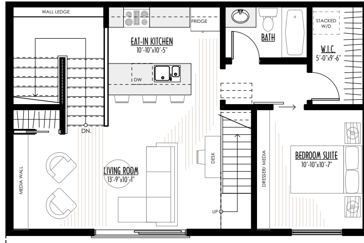
LEVEL 2 LIVING SPACE
