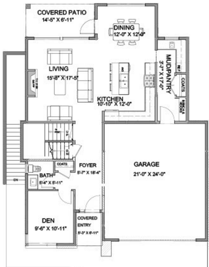
Main Floor Area: 1089 sqft
